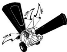
Figure 16: Lubrication Chart
